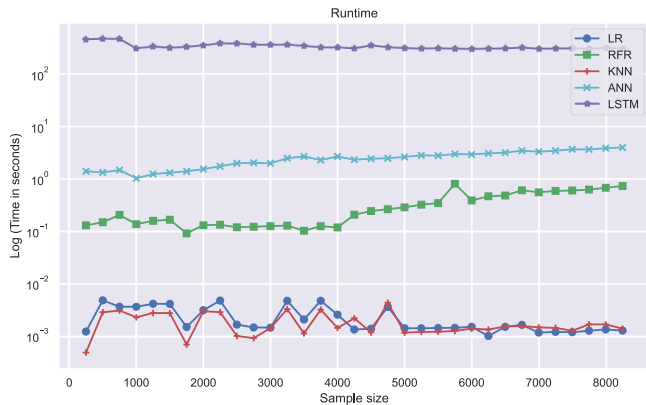
Fig. 9. Runtime analysis.
